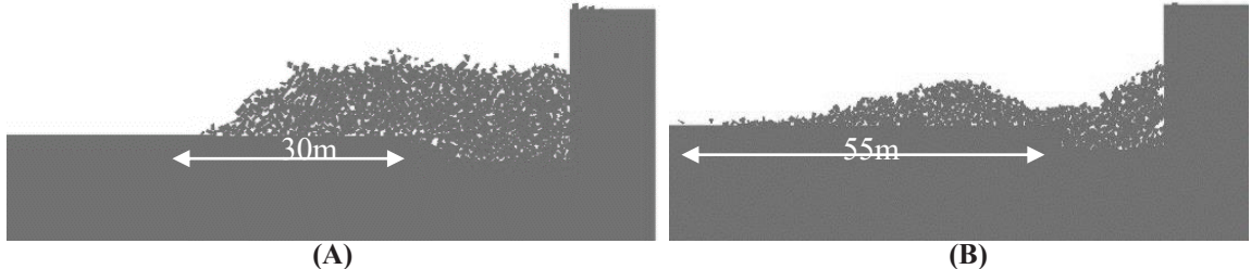
Figure 3. The final movement of fragmented rocks for two rows of blasting with the inter-row delay times of A: 17 ms and B: 50 ms
