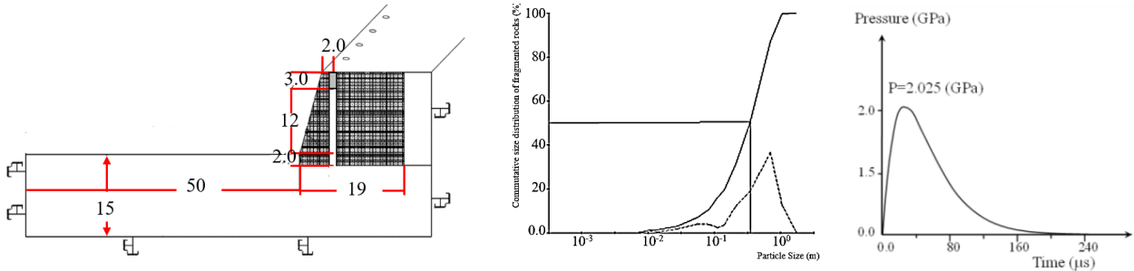
Figure 1. Model geometry, boundary conditions, size distribution, and blast puls loading in numerical modeling using UDEC
